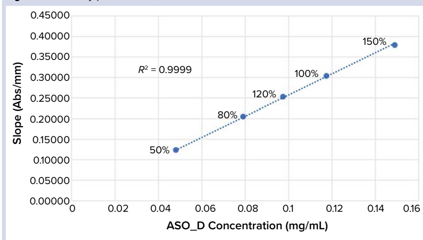
Figure 2: Linearity plot for ASO_D
